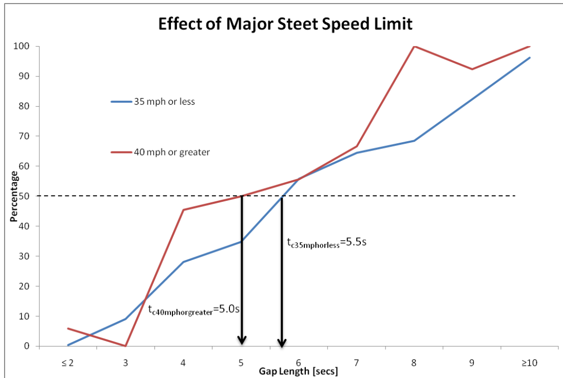
Figure 27. Effect of Major Street Speed Limit
