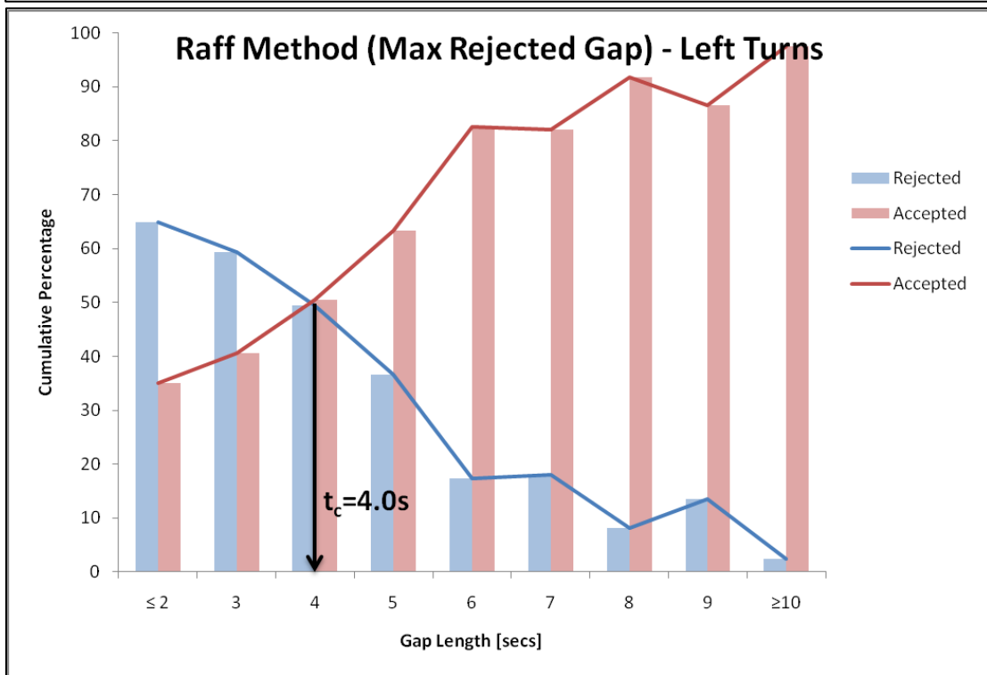
Figure 15. Raff Method (Max Gap Rejected Variation)
