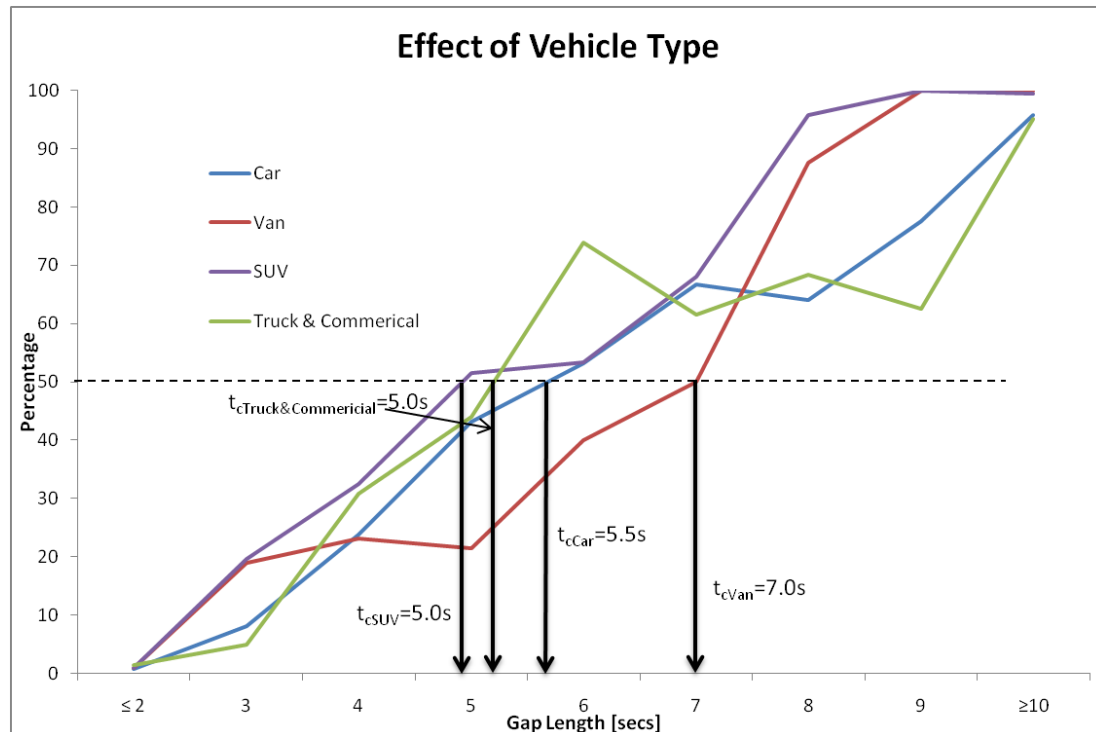
Figure 25. Effect of Vehicle Type
