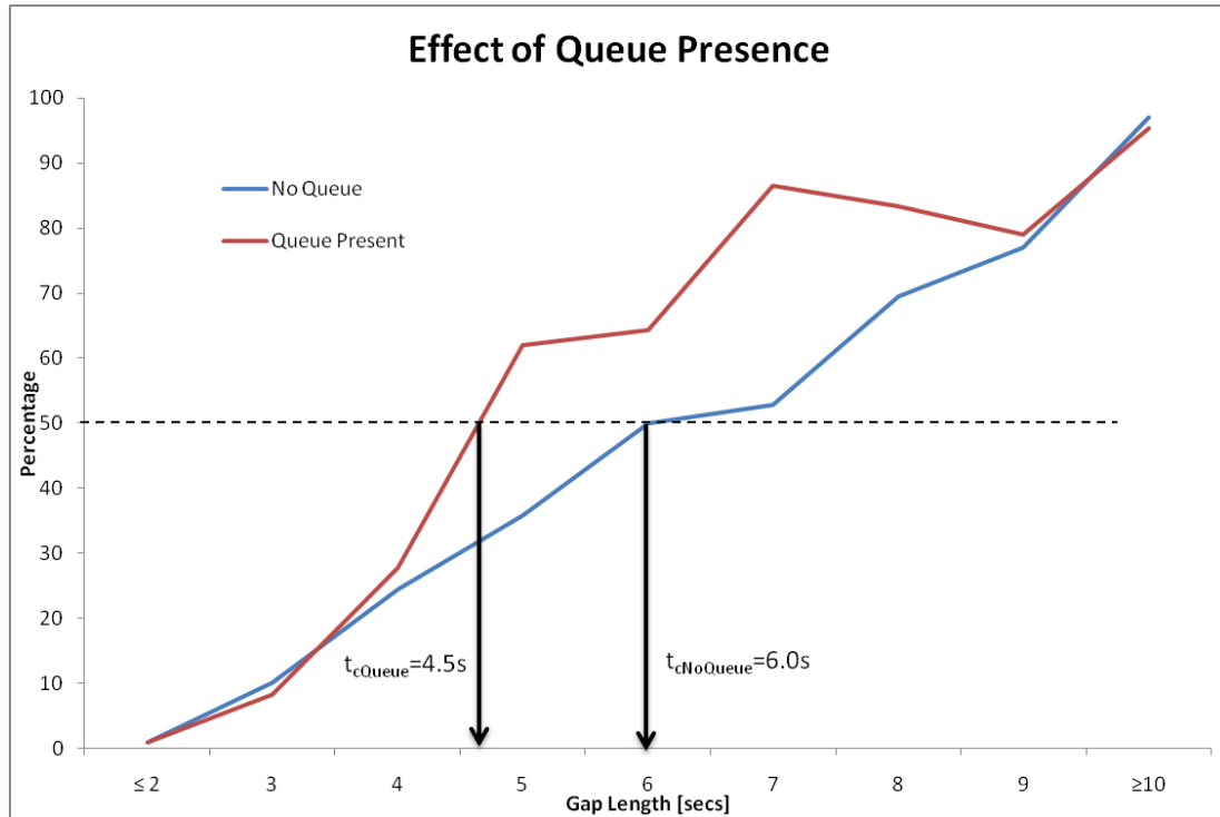
Figure 32. Effect of Queue Presence
