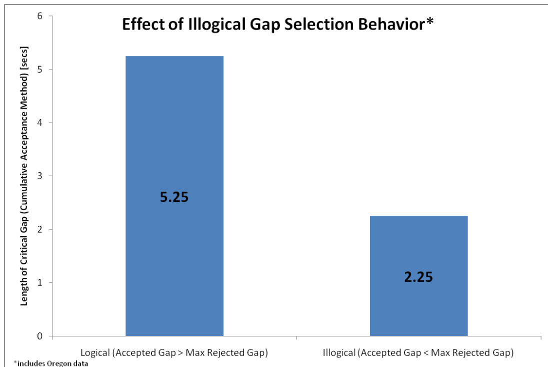
Figure 26. Effect of Illogical Gap Acceptance Behavior
